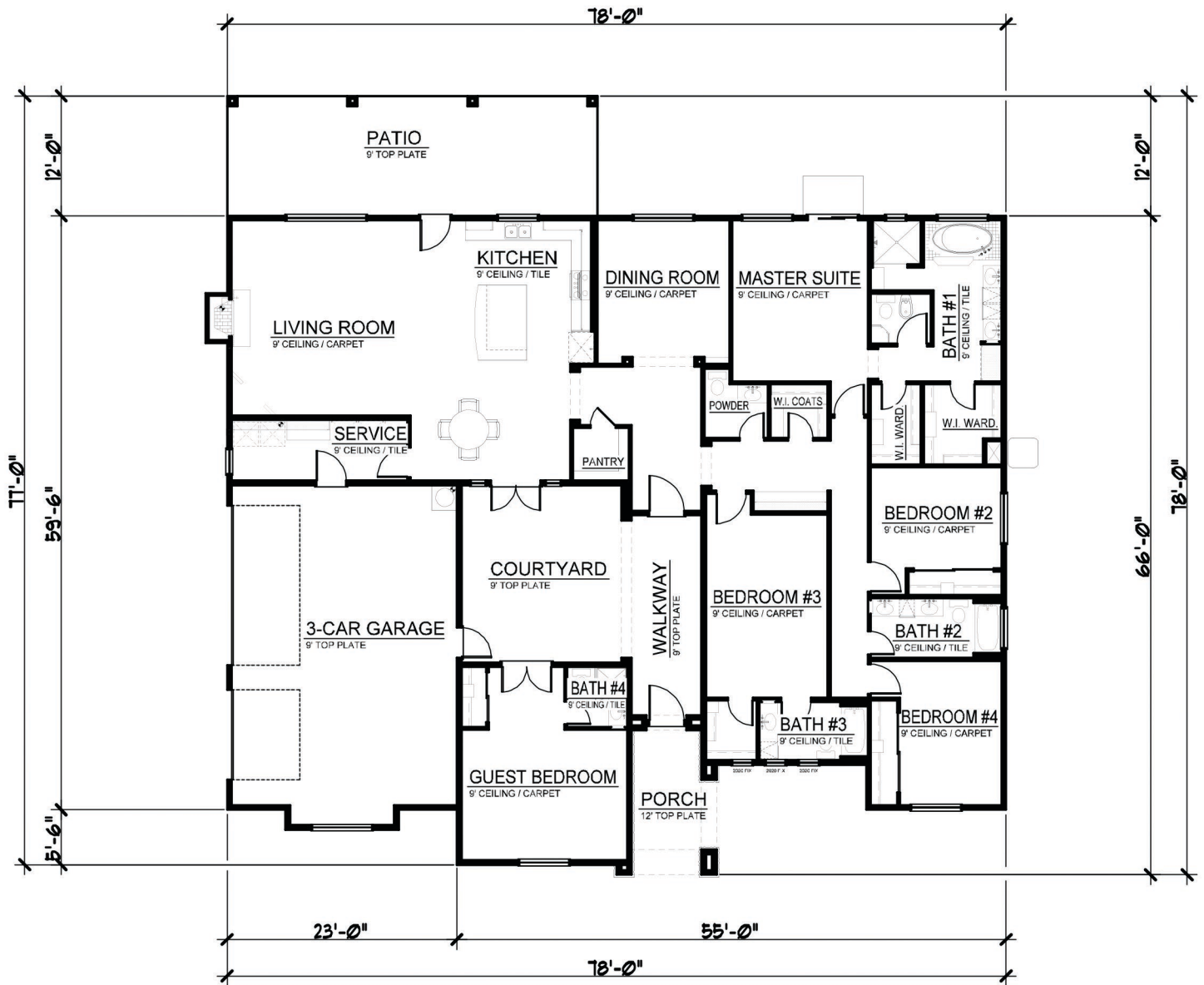
FLOOR PLAN
