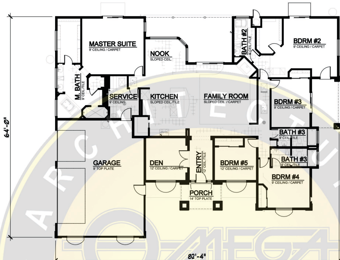
FLOOR PLAN
