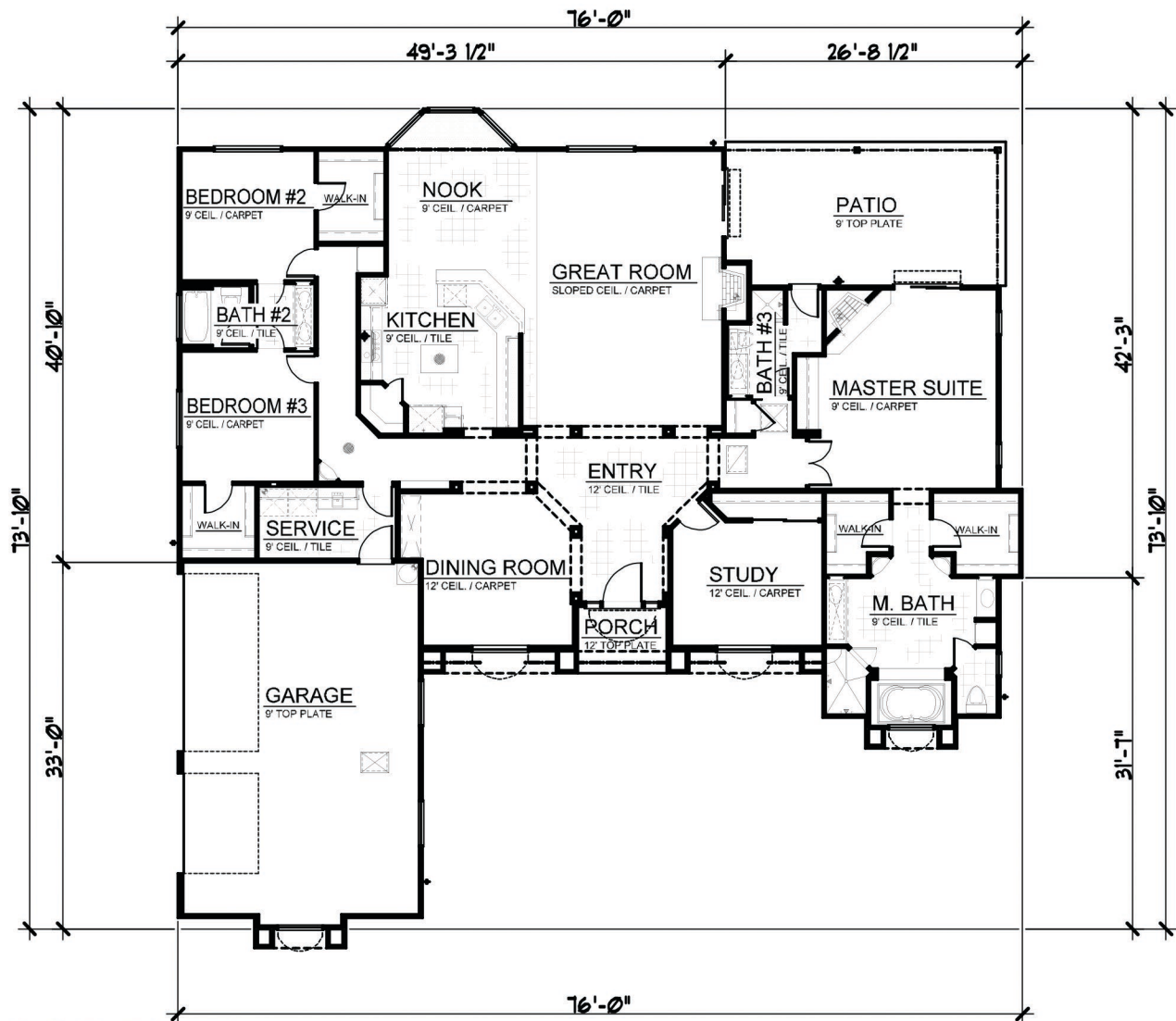
FLOOR PLAN
